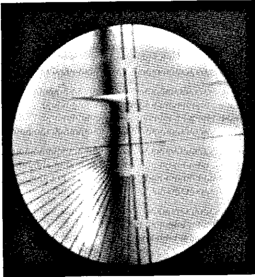
Figure 1 Photoelastic observation with Babinet compensator of a cross-section of a glass tube showing high tensile stress at the inner surface.
