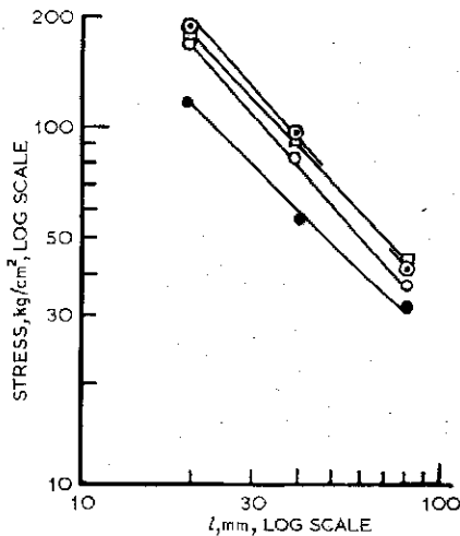
Figure 5 Relation between the distance l and the stress in the reference and neutron irradiated glasses after 1000 h of ultra-violet irradiation. Value of prior neutron irradiation: ○—○—○: 10^7 n/cm 2 ; ○—○—○: 10^{10} n/cm 2 ; □—□—□: 5.4 \times 10^{14} n/cm 2 ; ●—●—●: not irradiated.
