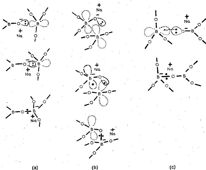
Figure 3 Processes of the structural change of borate glass by ultra-violet light caused by (a) excitation and elongation of B-O unit; (b) charge transfer in B-O unit; (c) photoionisation of non-bridging oxygen. -•-•-: orbital containing unpaired electron; - - - -: vacant p -orbital of boron; —: lone pair of oxygens; ●: electron.
