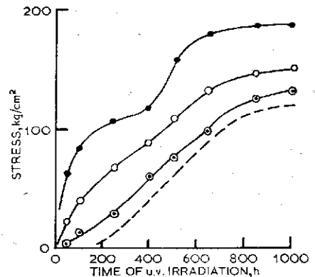
Figure 7 Kinetics of the stress build-up in glasses subjected to prior neutron irradiation of 5.4 \times 10^{14} neutrons/cm 2 and successive heating at 240° C for various times ( l = 20 mm). ○—○—○: 30 min; ○—○—○: 120 min; ●—●—●: not heated; - - - -: reference curve.
