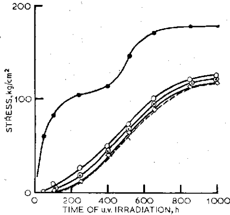
Figure 8 Kinetics of the stress build-up in glasses subjected to prior neutron irradiation of 5.4 \times 10^{14} neutrons/cm 2 and successive heating at 300° C for various times ( l = 20 mm). ○—○—○: 10 min; ○—○—○: 70 min; □—□—□: 150 min; ●—●—●: not heated; ---: reference curve.
